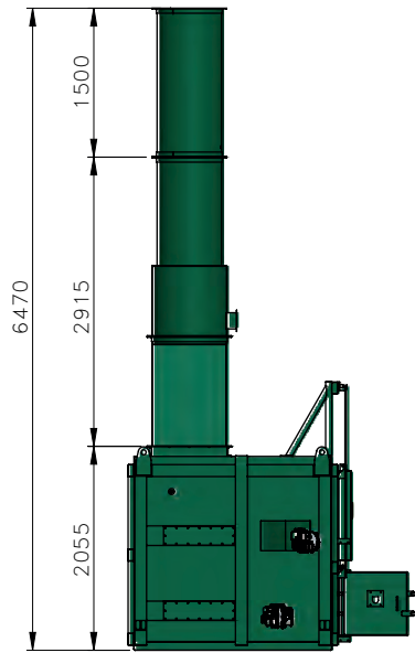
SIDE VIEW DOOR OPEN
