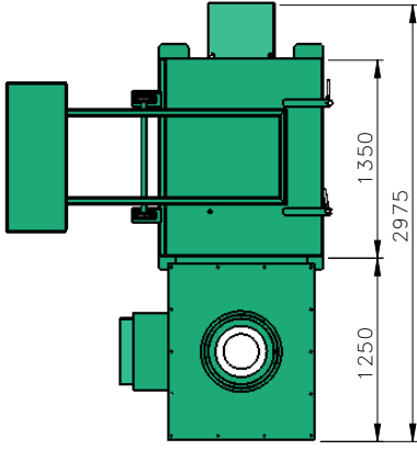
PLAN VIEW
